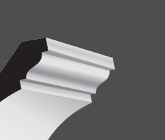
GEORGETOWN 1" x 8 3/8" x 12' P = 6-3/8"
